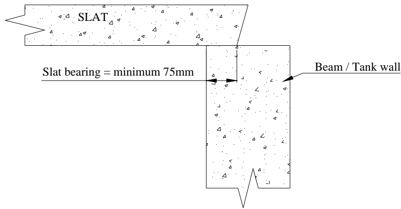
Figure 2: Diagram showing concrete slat bearing.
