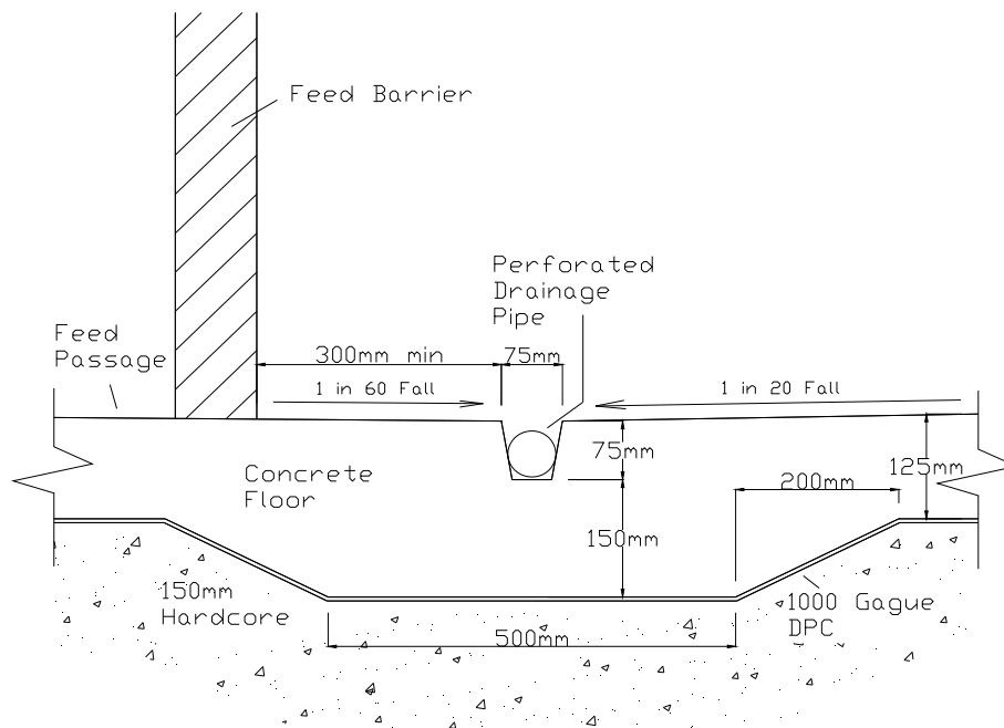
Figure 1 Construction of drainage channel
