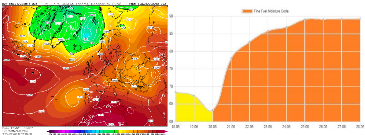
Fire Weather Data Courtesy of European Commission Copernicus System, European Centre for Medium Range Weather Forecasting and Met Eireann.
