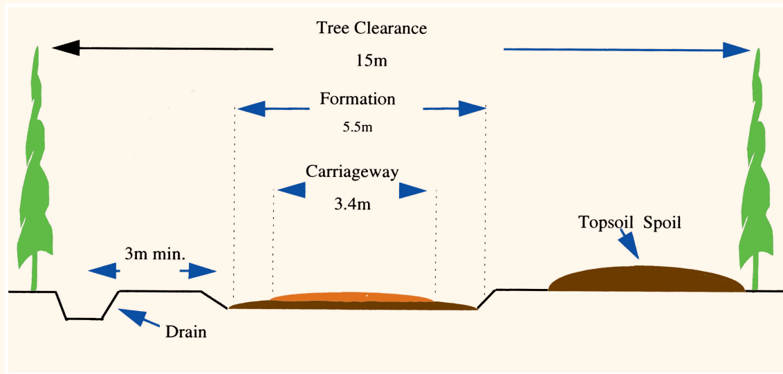
Figure 14. Typical road cross section.
