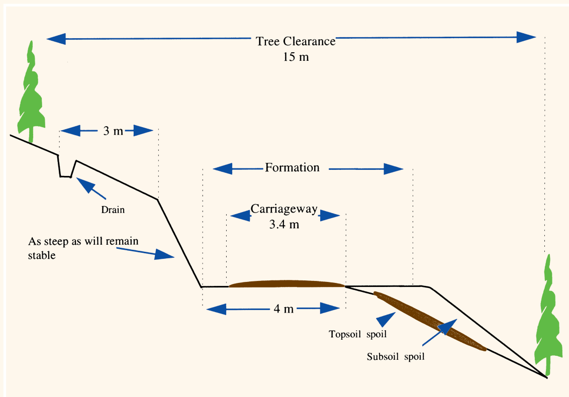
Figure 15. Typical cross section of road built on a slope
