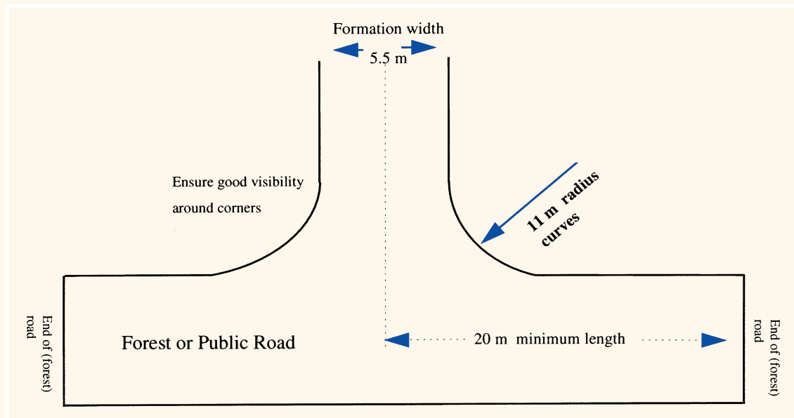
Figure 16. Diagram indicating curvature required for bellmouths onto public roads and internal turning bays or hammer heads.
